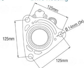
Drive Housing
