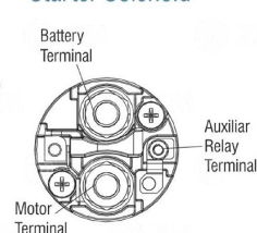
Starter Solenoid
